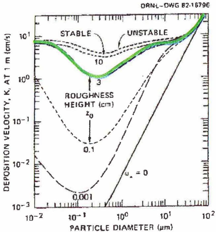
Figure A-1. Deposition velocity vs. particle diameter from Sehmel and Hodgson (1976) (friction velocity, U^* , of 100 cm/sec).
