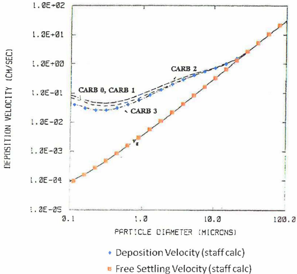
Figure C-2. Benchmarking of calculations by the Board's staff against results of EPA deposition velocity prediction methods outlined in Figure D-1 of EPA-454/R-94-015.
