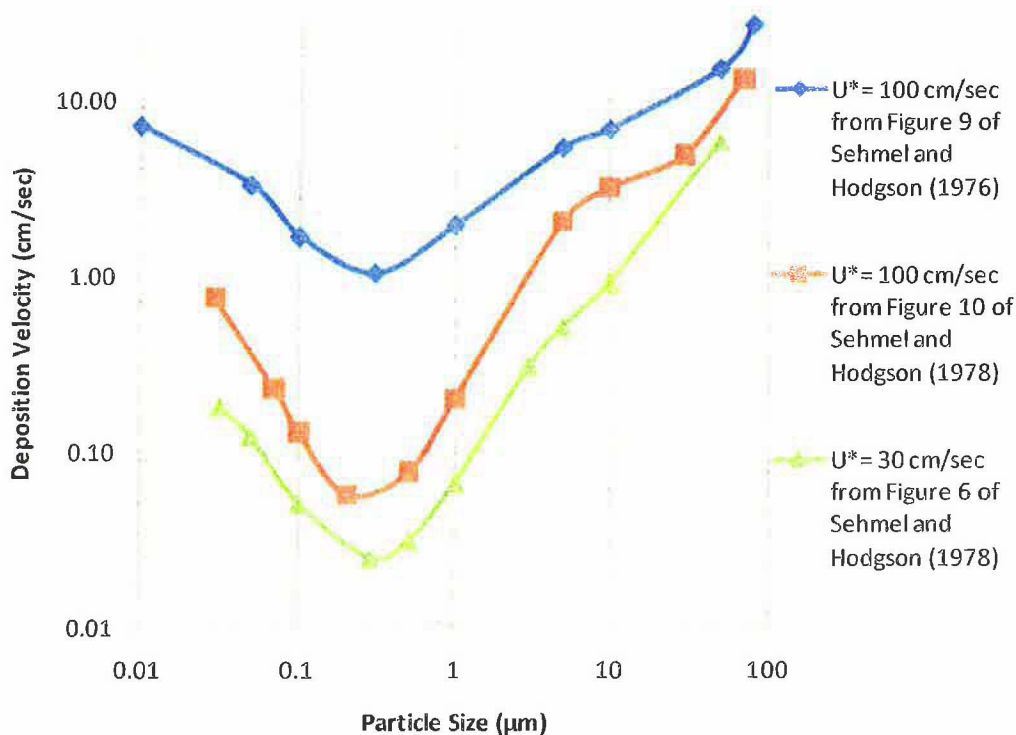
Figure 1. Selected deposition velocity curves from Sehmel and Hodgson (1976, 1978).
