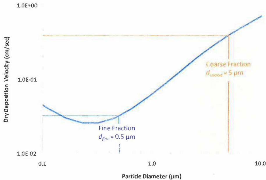
Figure 2. Example showing two particle-size bins for coarse and fine particles with a specific gravity of unity.
