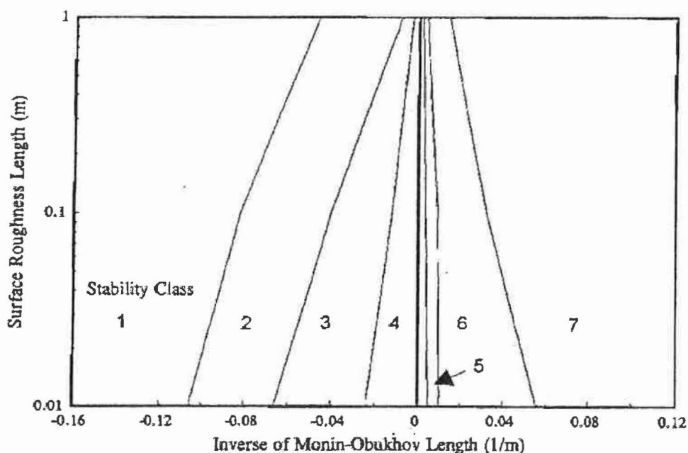
Figure C-1. Estimate of Monin-Obukhov mixing length under different atmospheric stability classes. 22
