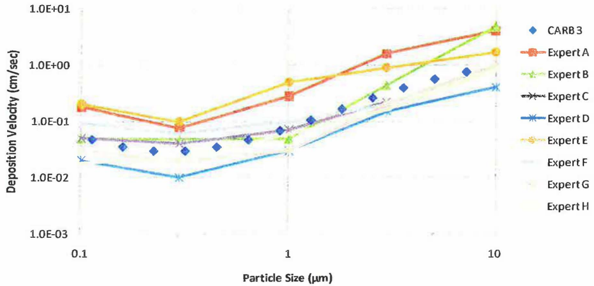
Figure 3. Comparison of CARB 3 deposition velocity calculations and NRC expert elicitation data corresponding to median quantiles at a wind speed of 4.5 mi/hr and surface roughness of 5 cm.
