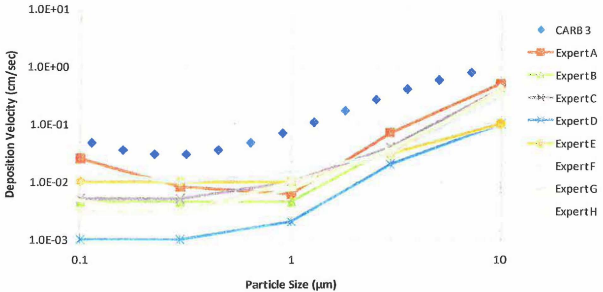
Figure 4. Comparison of CARB 3 deposition velocity calculations and NRC expert elicitation data corresponding to lower 5 percent quantiles at a wind speed of 4.5 mi/hr and surface roughness of 5 cm.
