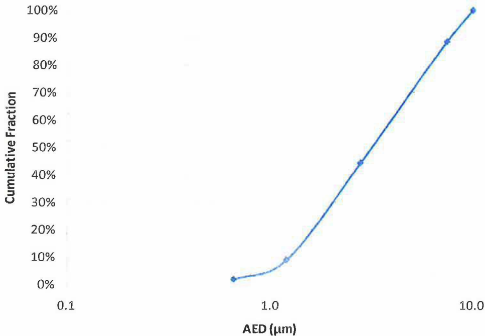
Figure B-1. Estimate of particle-size distribution in the respirable fraction for Hanford high-level waste.
