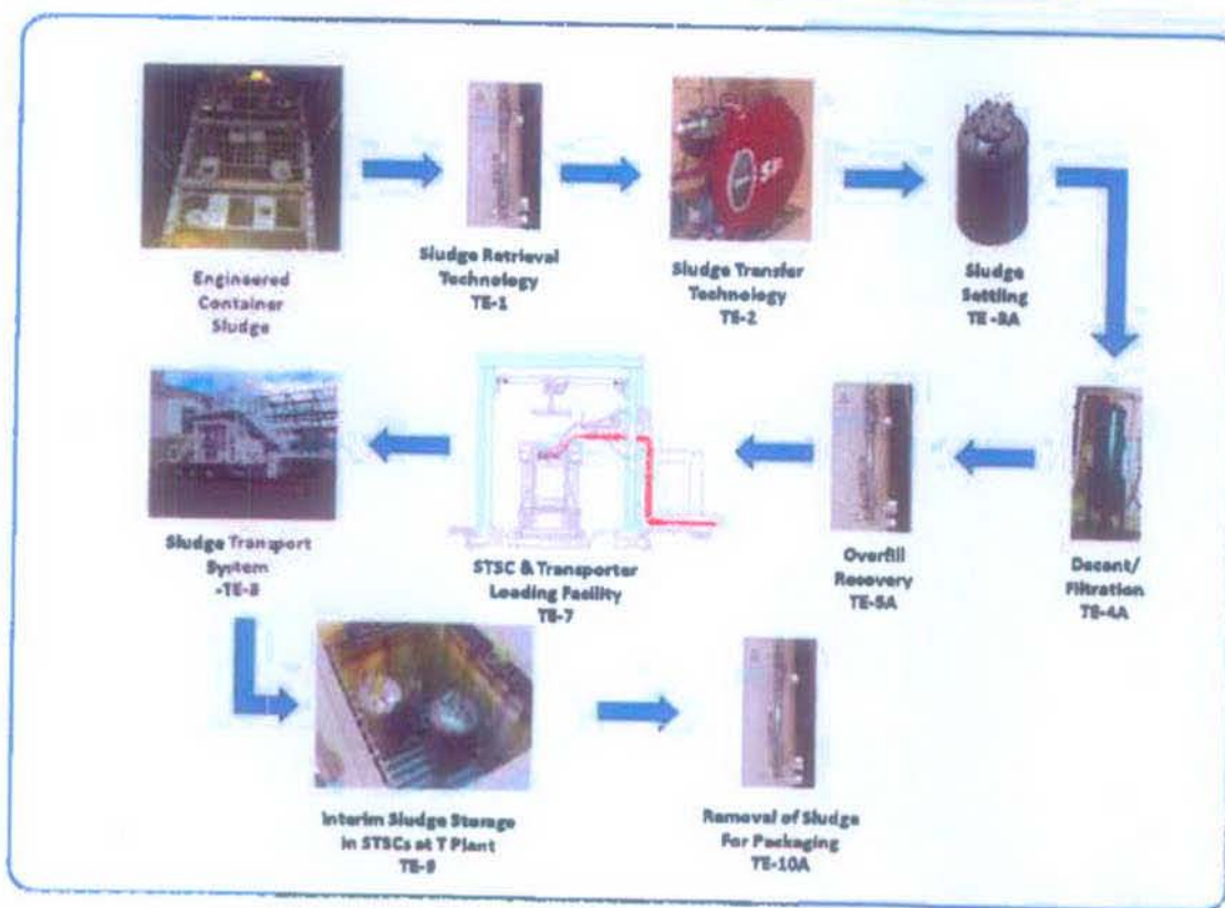
Figure 4-1, STP Phase 1 Material Handling/Process
