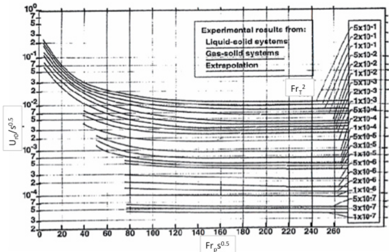
Figure 7-18. Molerus Diagram for Suspension Transport Data. Diagram can be obtained from both Selah (2002) and Molerus (1993)
