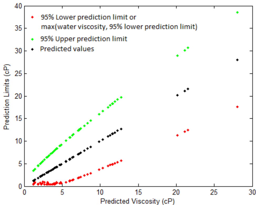
Figure 5-11. Lower and Upper Limits of 95% Prediction Intervals for the Data Points Used to Fit the Liquid-Viscosity Model
