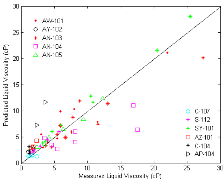
Figure 5-10. Predicted versus Measured Plot for the Data Used to Fit the Liquid-Viscosity Model in Equation 5-3
