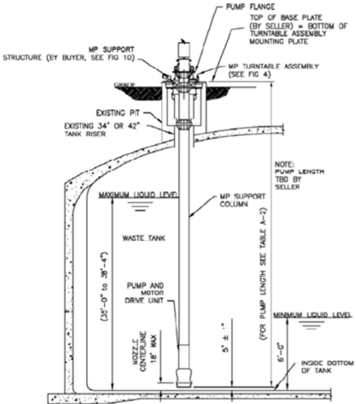
Figure 3-4. Mixer Pump Conceptual Arrangement (Pump Mounted on Pit)
