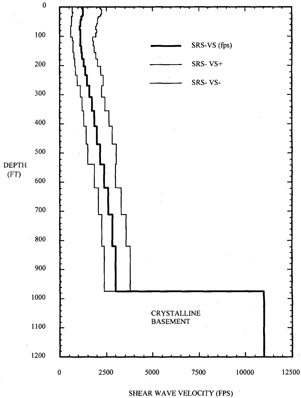
FIGURE 4 TYPICAL SHEAR WAVE VELOCITY PROFILE FOR SAVANNAH RIVER SITE File: HANFORD.VEL-SIGMA.CRD
