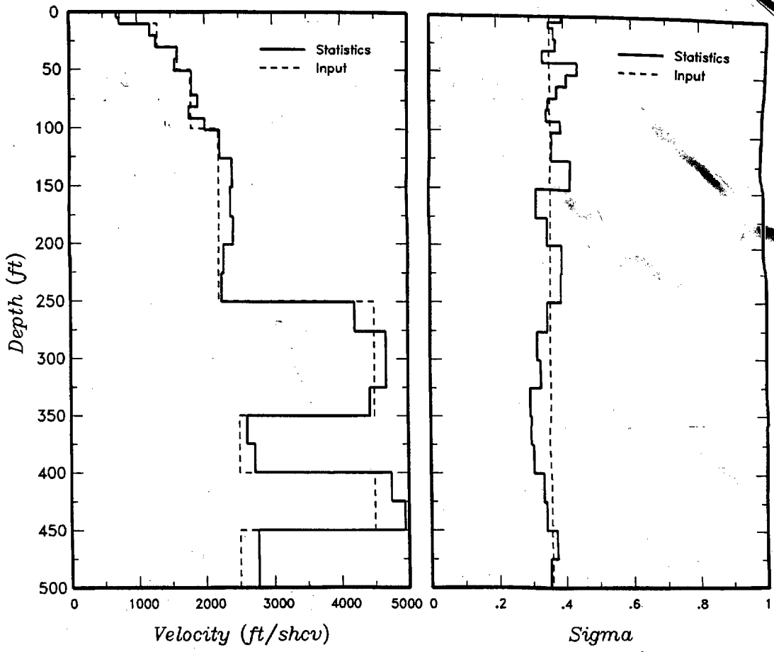
Figure 19. Comparison of Statistics of Randomized Hanford P3 Soil Velocity Profiles to Target Values for the California Soil Velocity Correlation Model.
