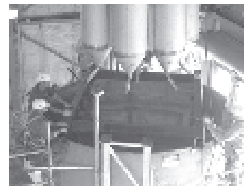
Pulse Jet Mixers at the Waste Treatment Plant located at the Hanford Site.
