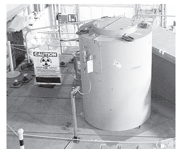
Interior view of Molten Salt Reactor Experiment facility located at the Oak Ridge National Laboratory.
