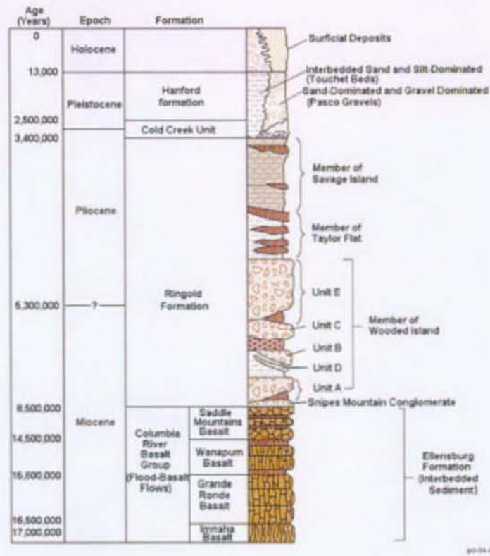
Figure 2.1.2. Generalized Stratigraphy of the Hanford Site and Waste Treatment Plant
