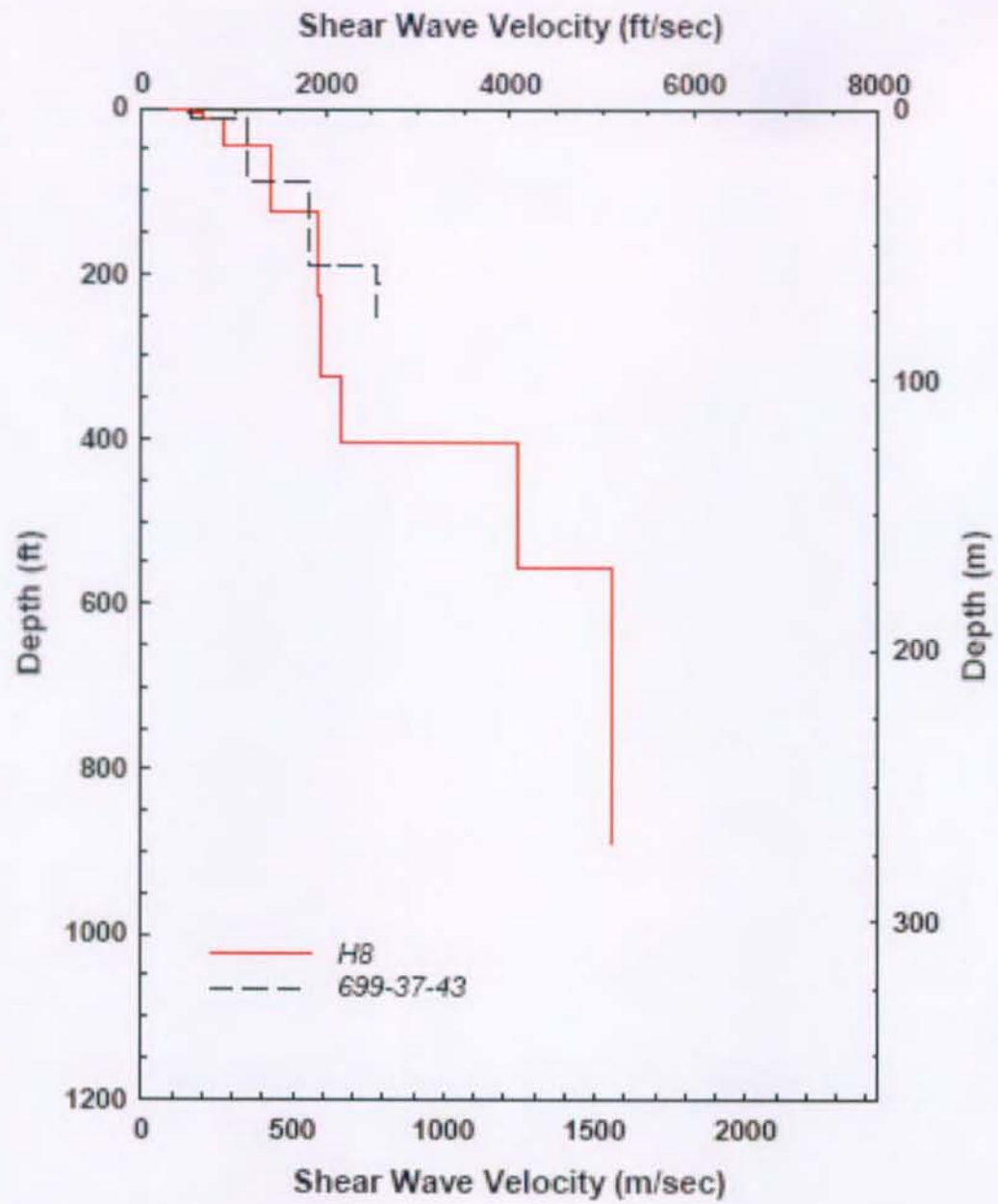
Figure 2.3.5.4. Comparison of SASW Profile H8 and Downhole Log at Site 8
