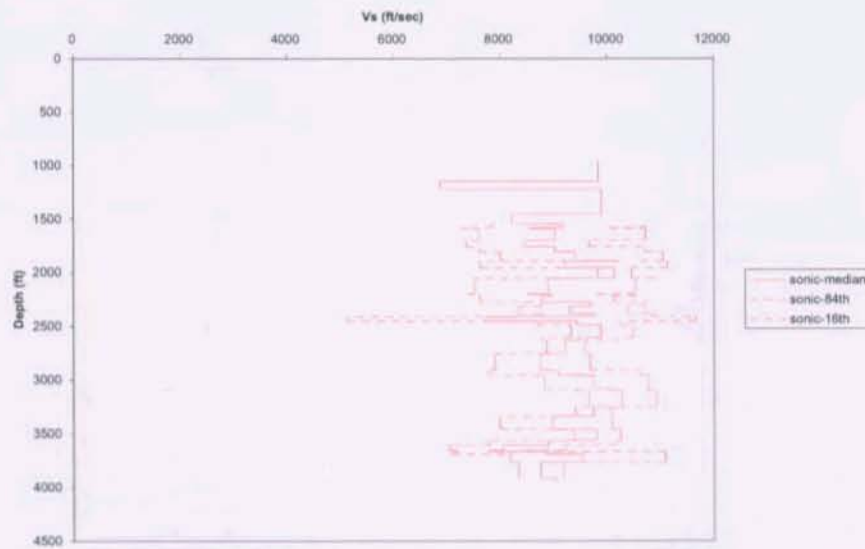
Figure 2.5.11. Fractile Basalt S-Wave Model Based on P-Wave Sonic Logs in Deep Basalts
