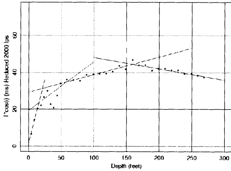
WTP Borehole BD-23
