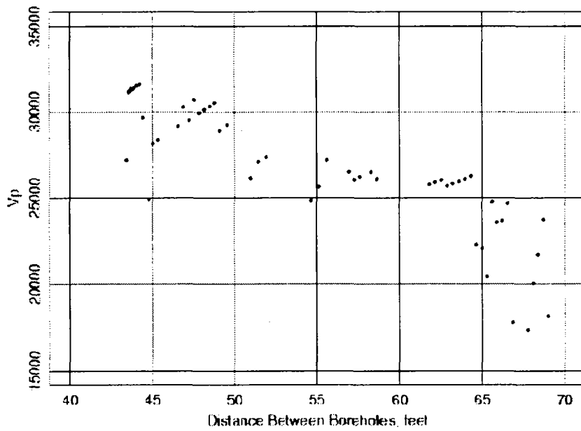
Figure 2.4.2.7. Correlation of V_p with Cross-Borehole Distance
