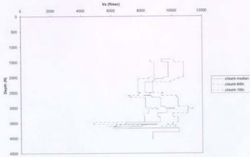
Figure 2.5.12. Fractile Basalt S-Wave Model Based on P-Wave Checkshot Surveys in Deep Basalts
