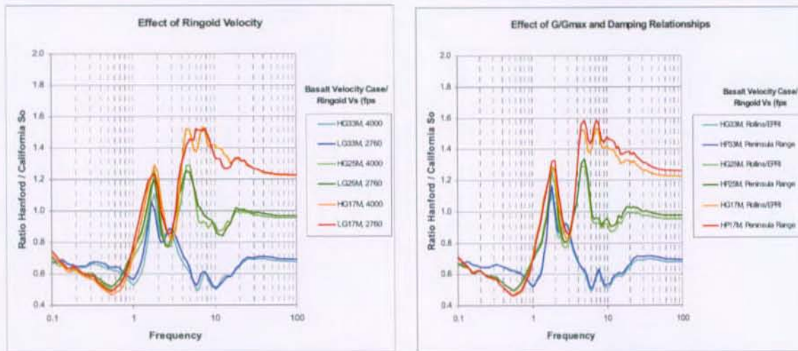
Figure 3.3.7. Effect of Alternative Ringold Velocities and Soil Modulus Reduction and Damping Relationships on Response Spectral Ratio (Waste Treatment Plant/California)
