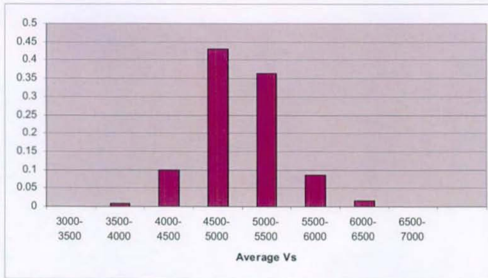
Figure 3.2.13. Distribution of Average Vs in Saddle Mountains Basalt and Interbeds Resulting from Logic Tree Weighting
