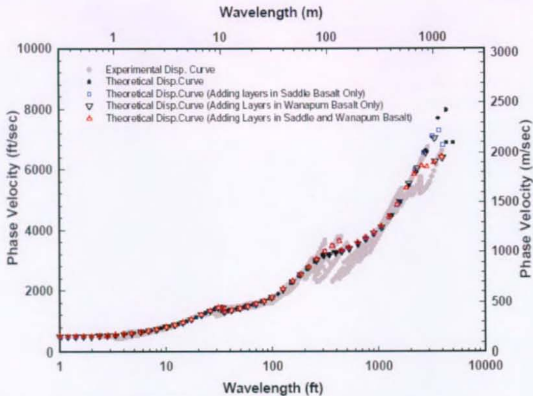
Figure 2.4.4.5. Comparison of SASW Dispersion Curve at Site 10 to Model of Basalts and Low-Velocity Interbedded Layers
