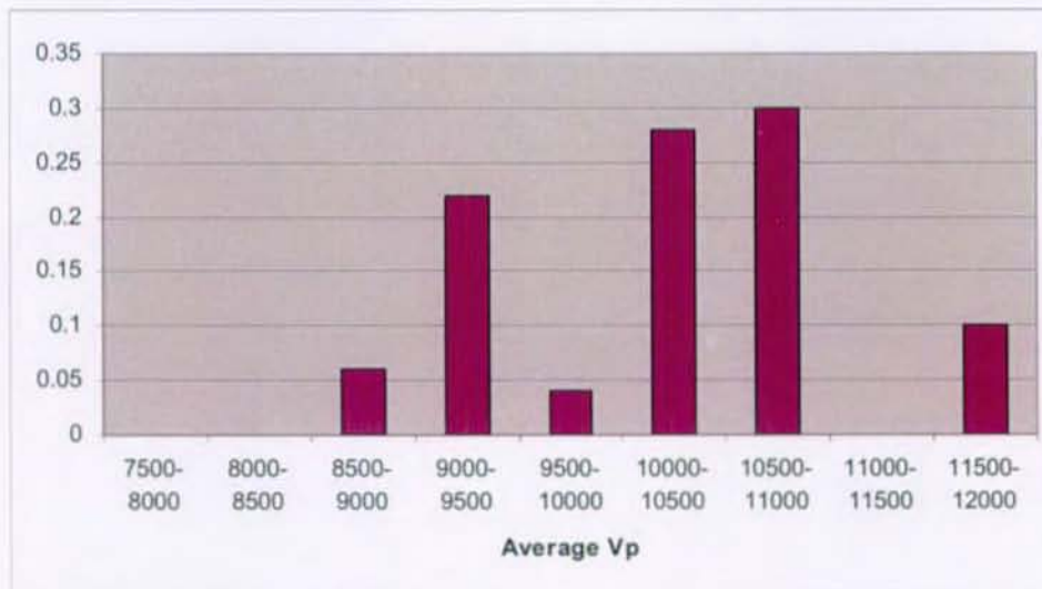
Figure 3.2.8. Distribution of Weights of Average Vp in the Basalt and Interbeds
