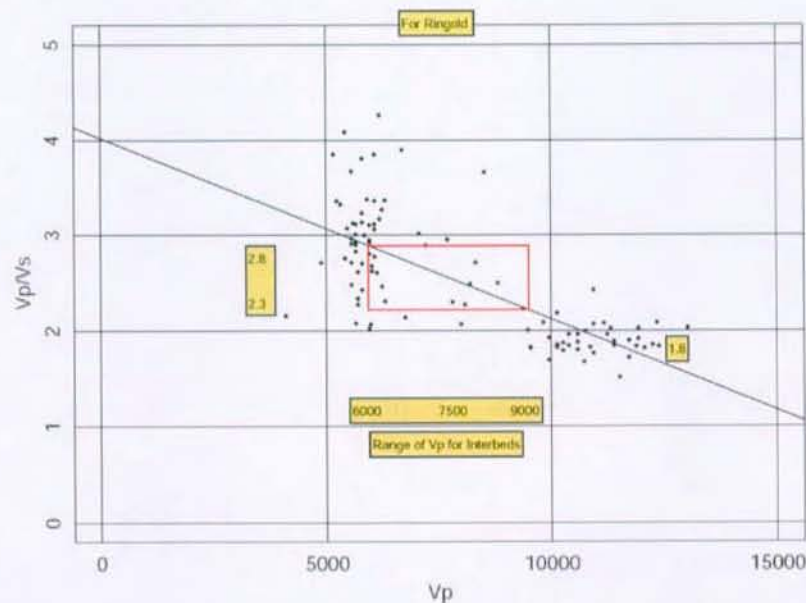
Figure 3.2.9. Velocity Ratio V_p/V_s Versus V_p in the Ringgold Compared to the Range of V_p in the Interbed Logic Tree
