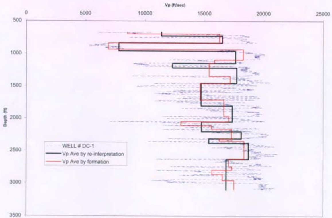
Figure 2.4.1.3. Comparison of Birdwell DC-1 P-Wave Sonic Log, Reinterpreted Profile, and Profile Controlled by Stratigraphic Formation
