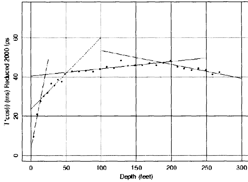
Figure 2.3.2.4. Reinterpretation of Shannon & Wilson Downhole Data from BD-47
