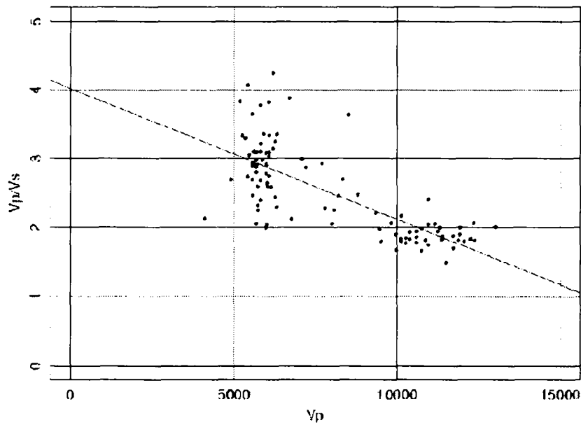
Figure 2.4.3.3. V_p/V_s Ratios from Ringold Formation Versus V_p . The regression equation that resulted was V_p/V_s = 4.02 - 0.19 \cdot 10^{-3} \cdot V_p(\text{fps}) . The resulting standard error was 0.44 after regression and 0.64 before.
