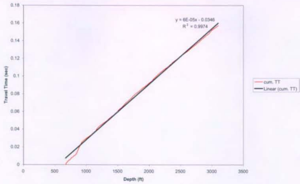
Figure 2.4.1.2a. Birdwell DC-1 Cumulative P-Wave Vertical Travel Time
