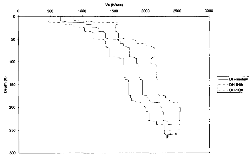
Figure 2.5.3. Fractile S-Wave Model of WTP Vicinity Sands and Gravels Based on Downhole Seismic Surveys
