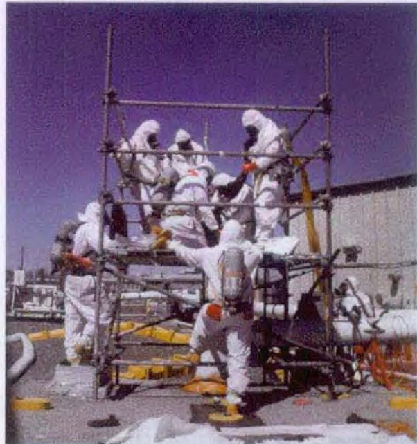
Replacing an In-Tank Video Camera in Tank C-103 To Support Waste Retrieval Activities
